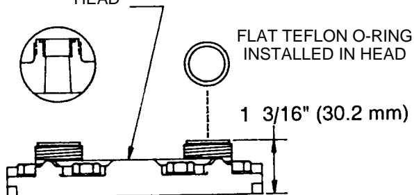
ROTOLOCK HEAD
